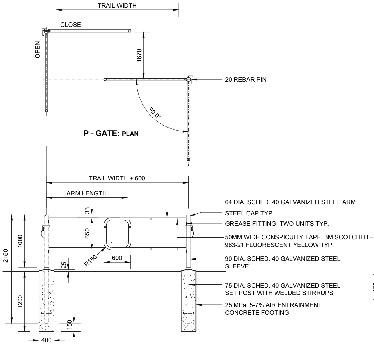
P - GATE: ELEVATION / SECTION
